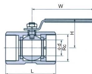
QZ11F female threaded one pieces ball valve
