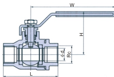
QL11F female threaded two pieces ball valve
