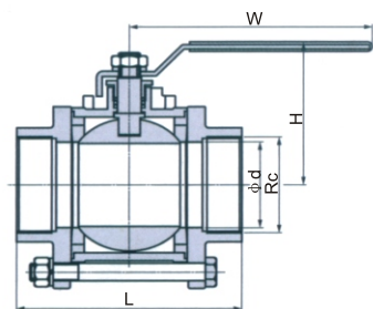
QS11F female threaded three pieces ball valve
