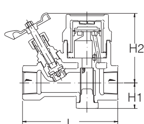
YSP - 1 Type Attachment of a bypass valve
