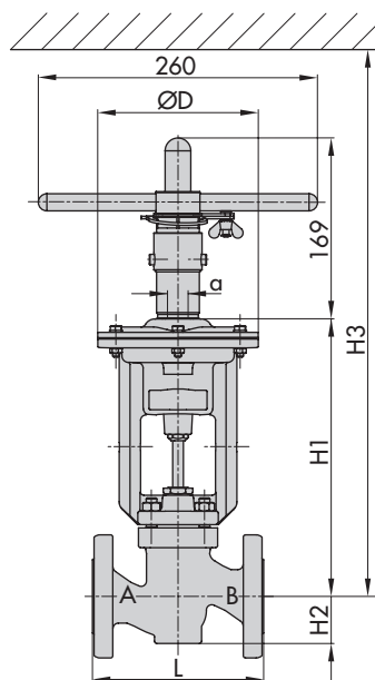
Type 3351 with manual override
