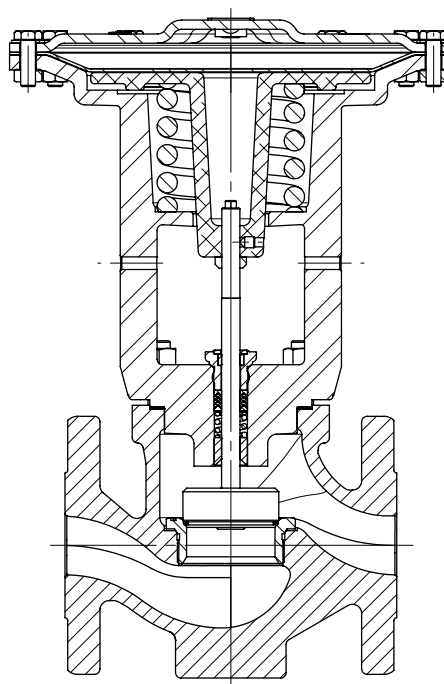
Fig. 5: Type 3351 Pneumatic On/off Valve · Fail-open version
