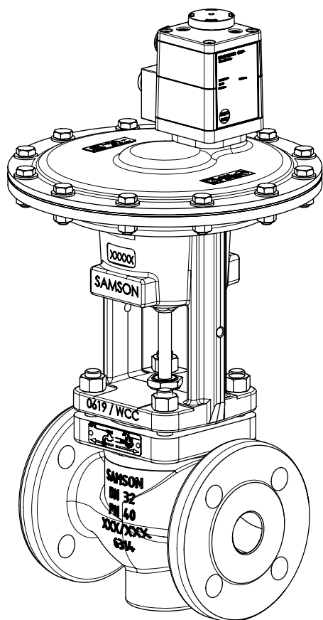
Fig. 3: Type 3351 with directly attached solenoid valve
