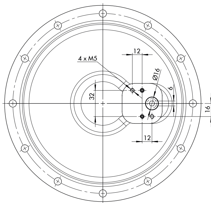
Adapter plate with NAMUR interface
