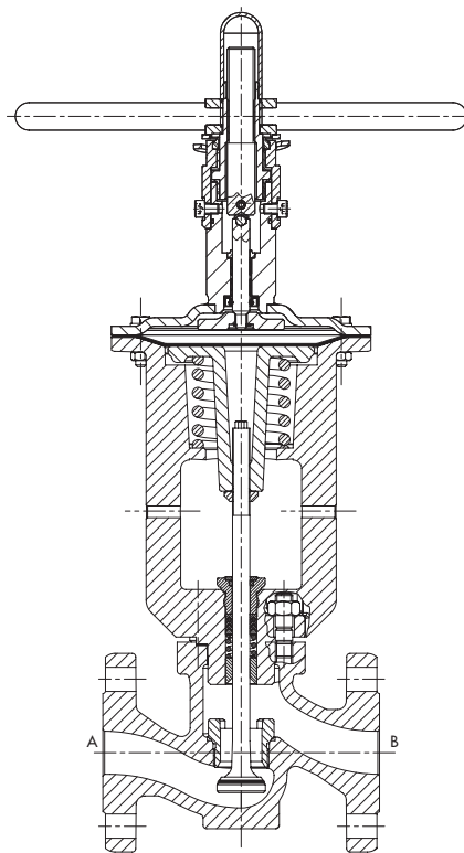
Fig. 4: Type 3351 Pneumatic On/off Valve with manual override Fail-close version
